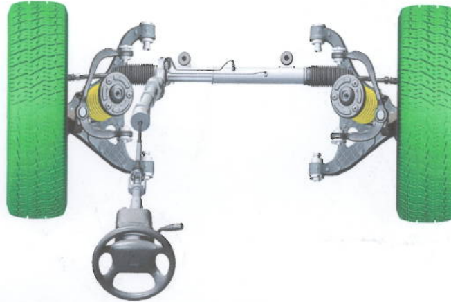
Total Front Toe
